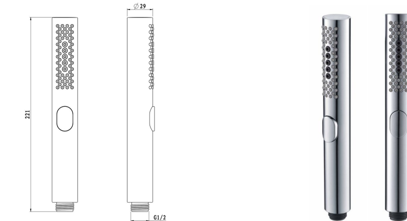
MMHST3 - Tubular hand shower - flow rate - maximum pressure rating: 9 Bar
